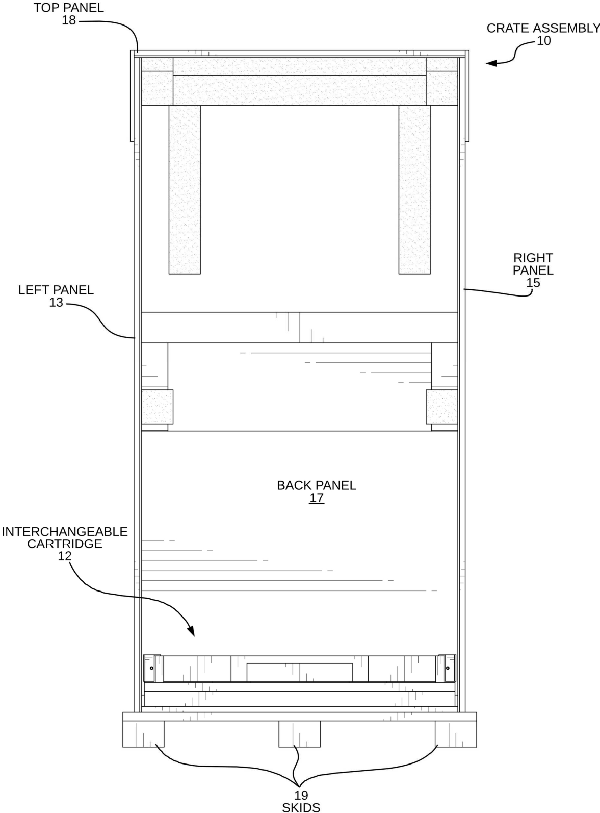
FRONT VIEW OF SERVER RACK CRATE FIG. 2
